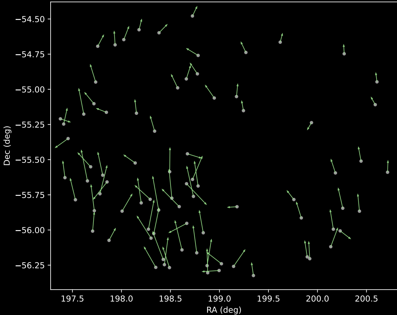
GALAH DR4 Cluster 5 Proper Motion Vectors (n=81)
