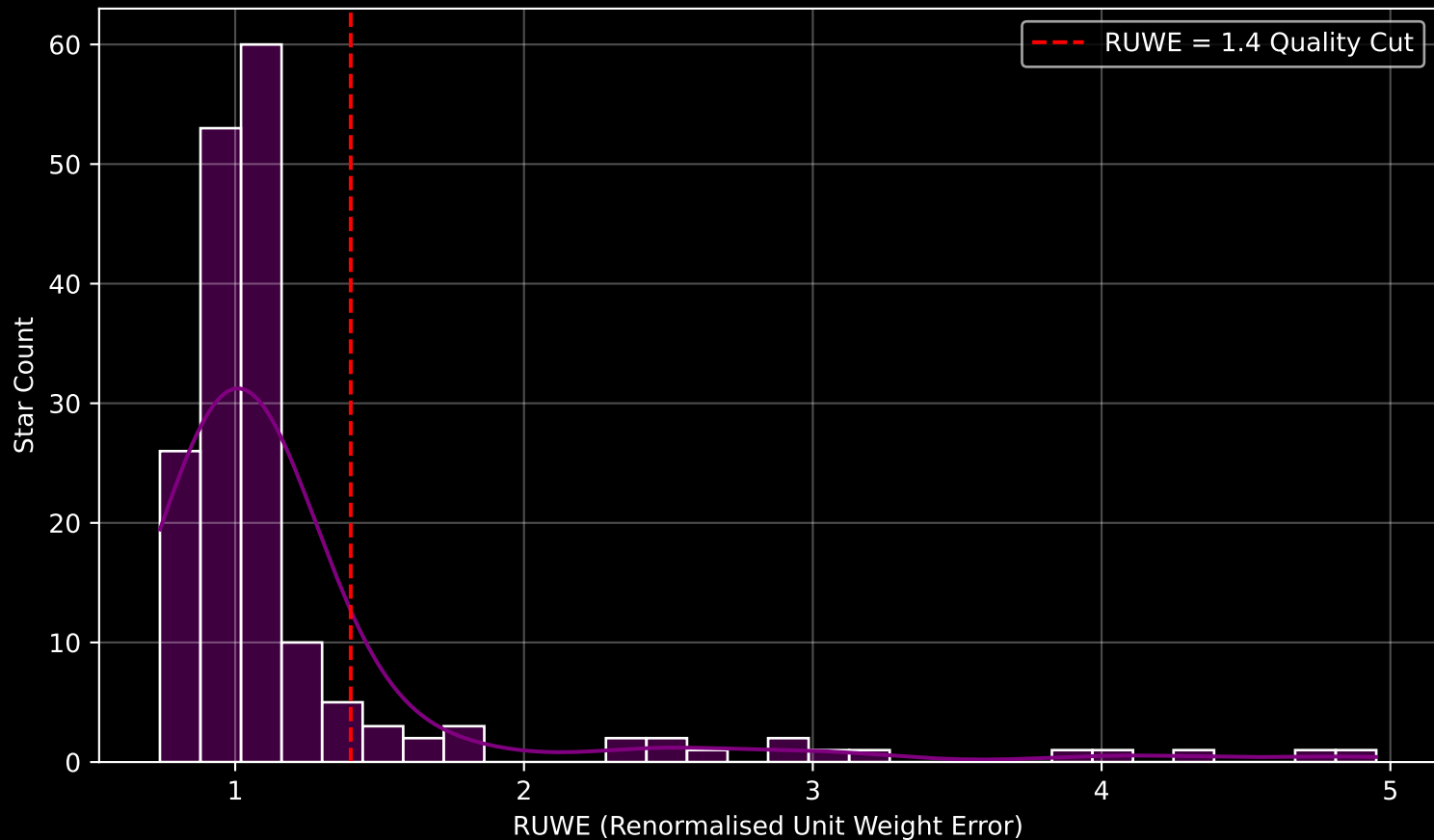
GALAH DR4 Field [7222] RUWE Distribution (n= 176)
