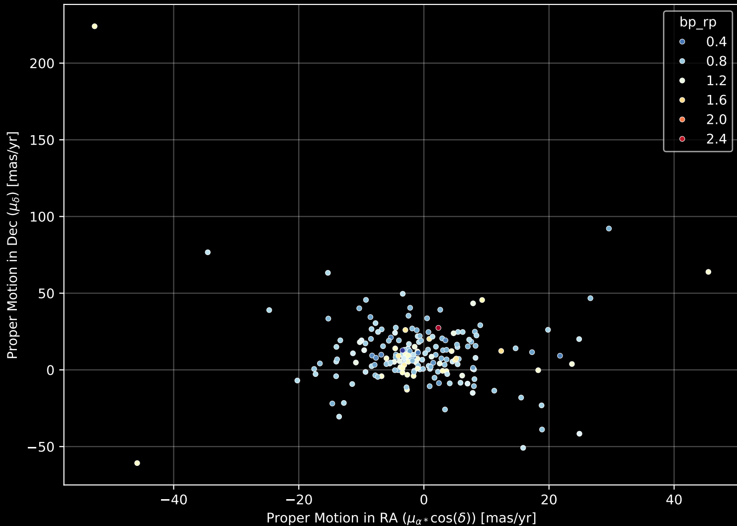
GALAH DR4 Field: [7222] Proper Motion Diagram (n= 191)
