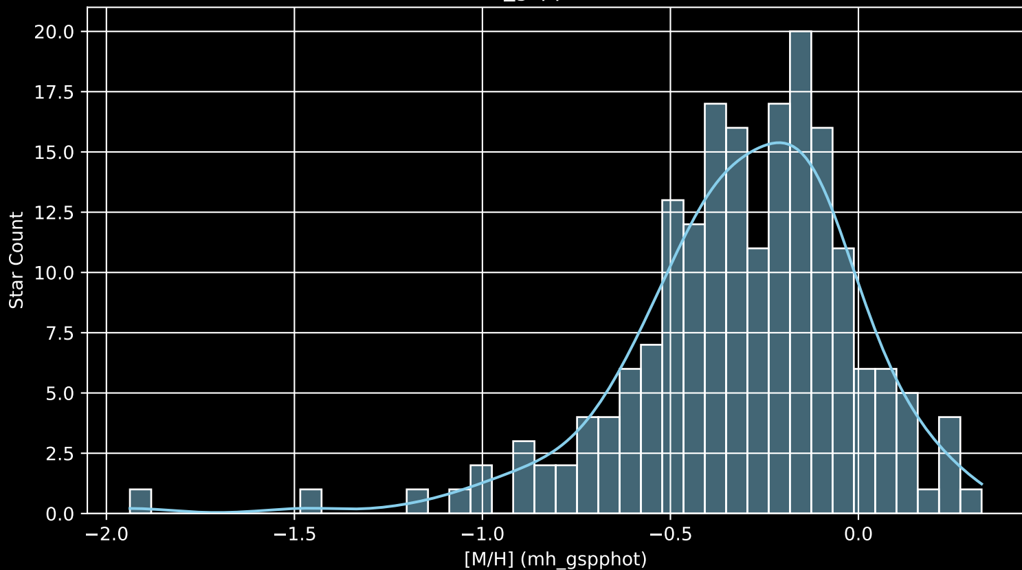
GALAH DR4 Field: [7222] [M/H] (mh_gspphot) (n= 190)
