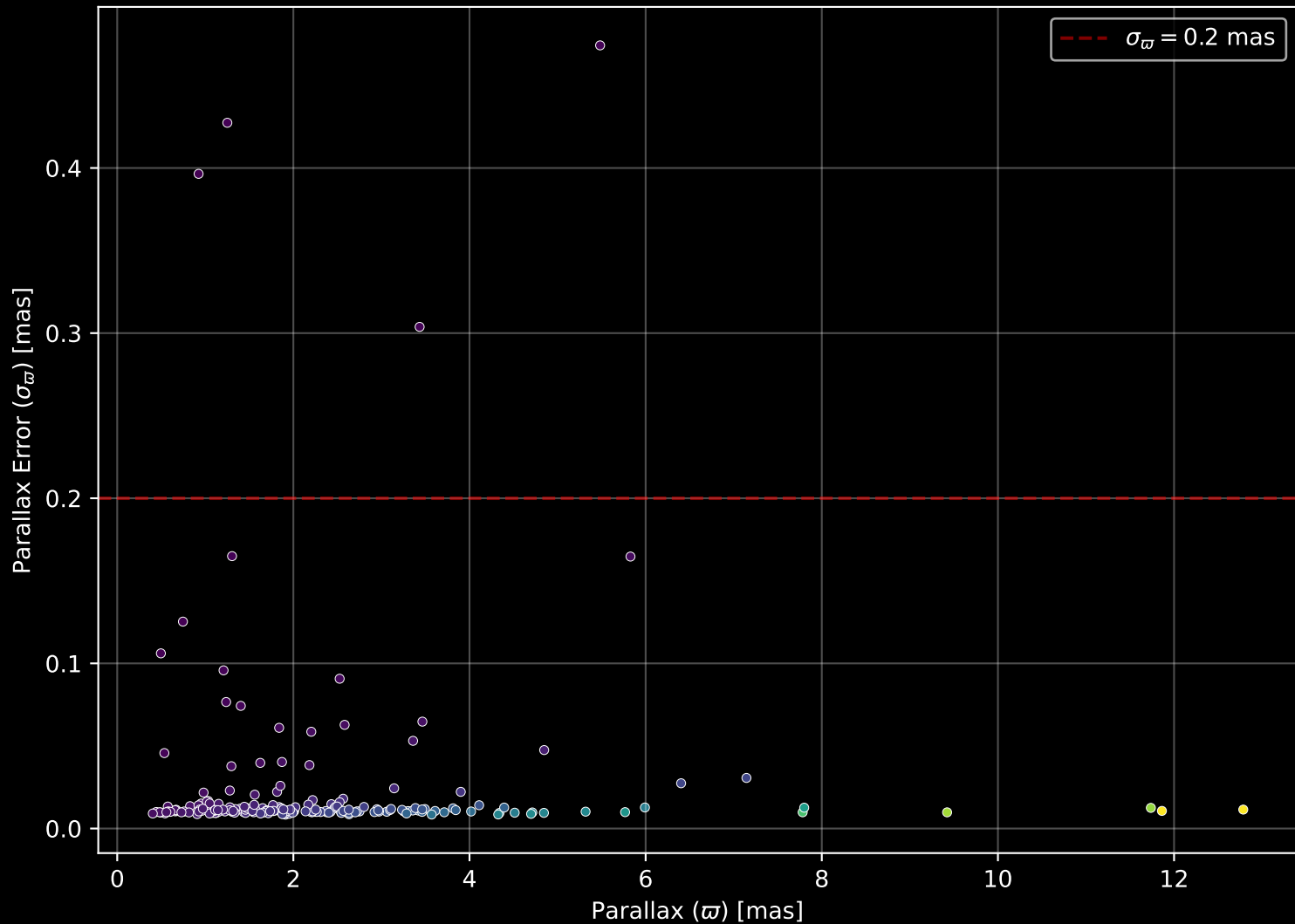
GALAH DR4 Field: [7222] Parallax Quality (n= 191)
