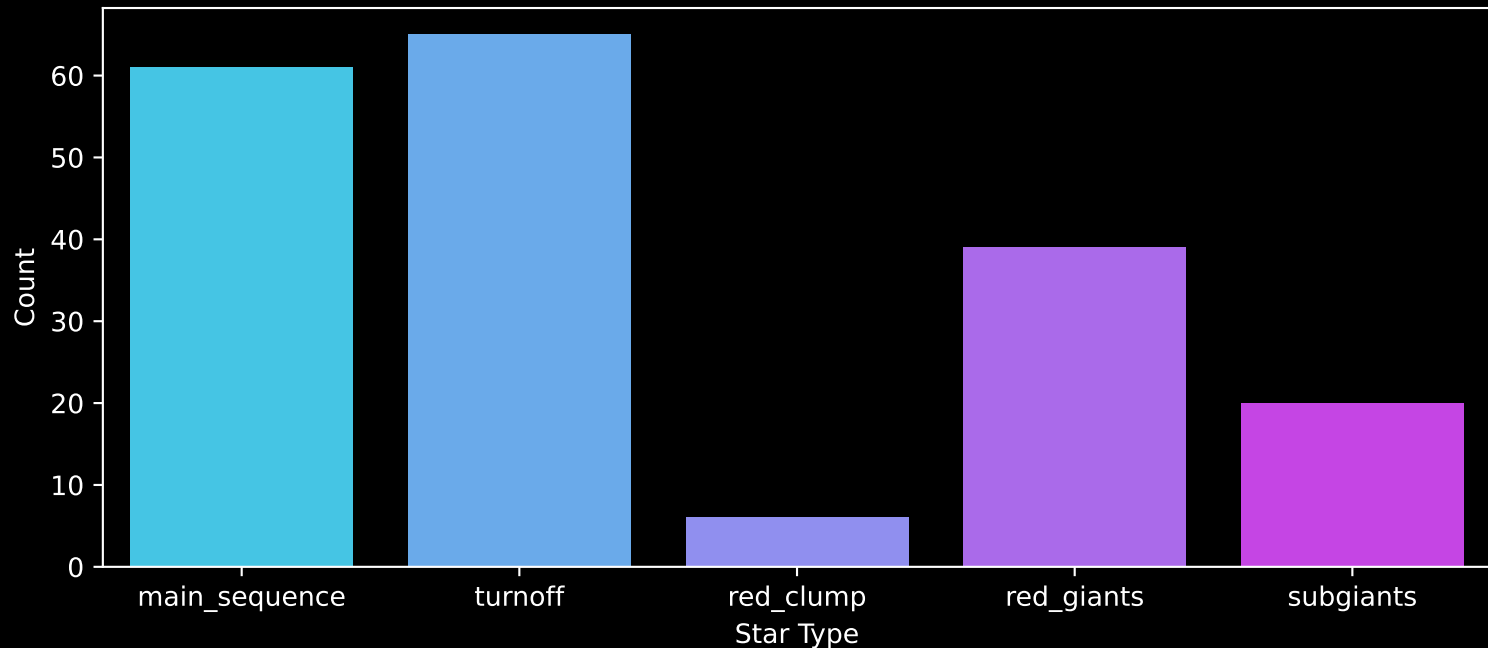
GALAH DR4 Field: [7222] Count plot of Star Type
